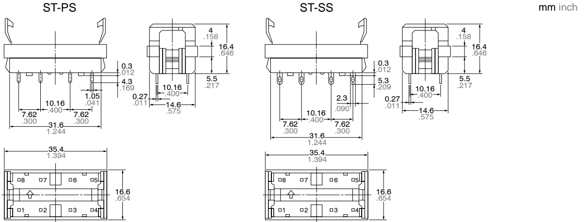
ST-PS PC board terminal socket
