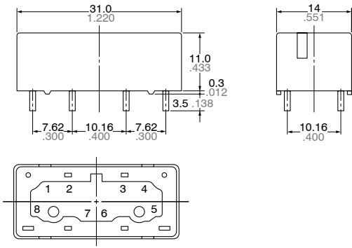
General tolerance: \pm 0.2 \pm 0.008 PC board pattern (Copper-side view)
