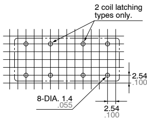
Tolerance: \pm 0.1 \pm 0.004
