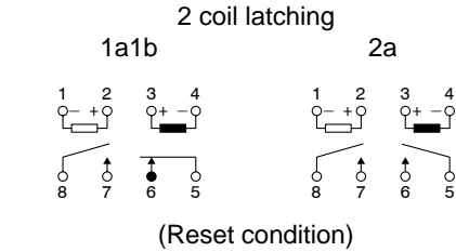
Diagram shows the "reset" position when terminals 3 and 4 are energized. Energize terminals 1 and 2 to transfer contacts.
