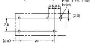
Mounting Holes (Bottom View)
