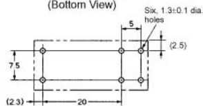
Mounting Holes (Bottom View)
