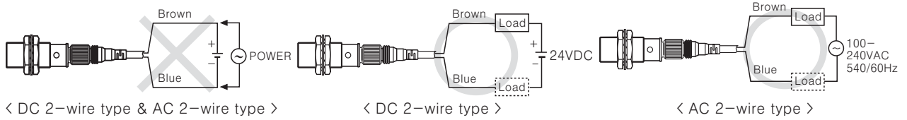
< DC 2-wire type & AC 2-wire type >
