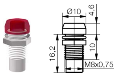
Blende Form A Lens Head Form A Typ / type
