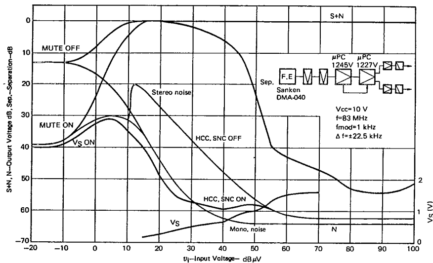
Fig. 14 Overall Characteristics
