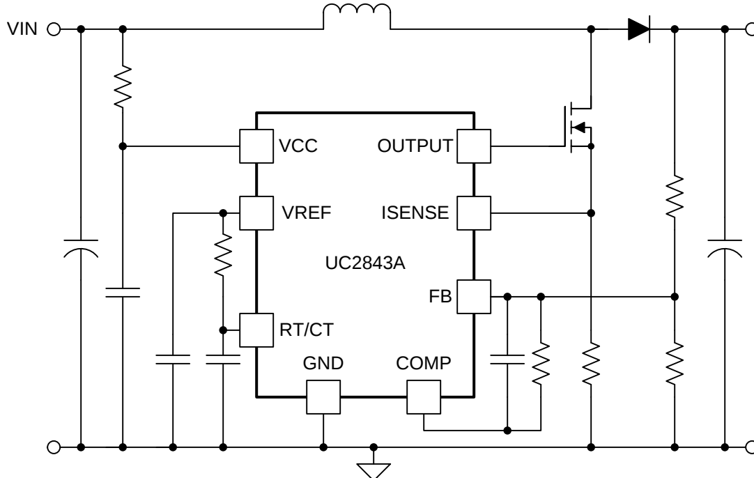
Simplified Application Diagram
