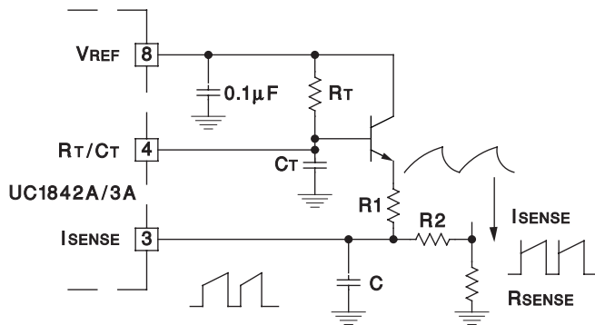
Figure 9. Slope Compensation
