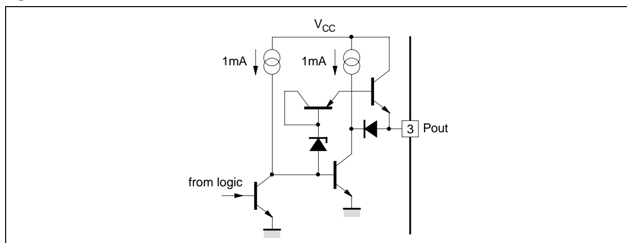
Figure 7 : Electrical Schematic
