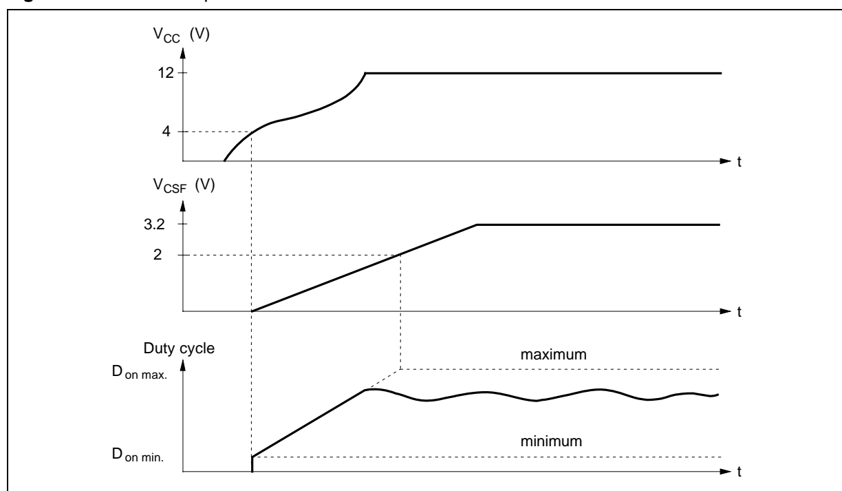
Figure 6 : Soft-Start Sequence
