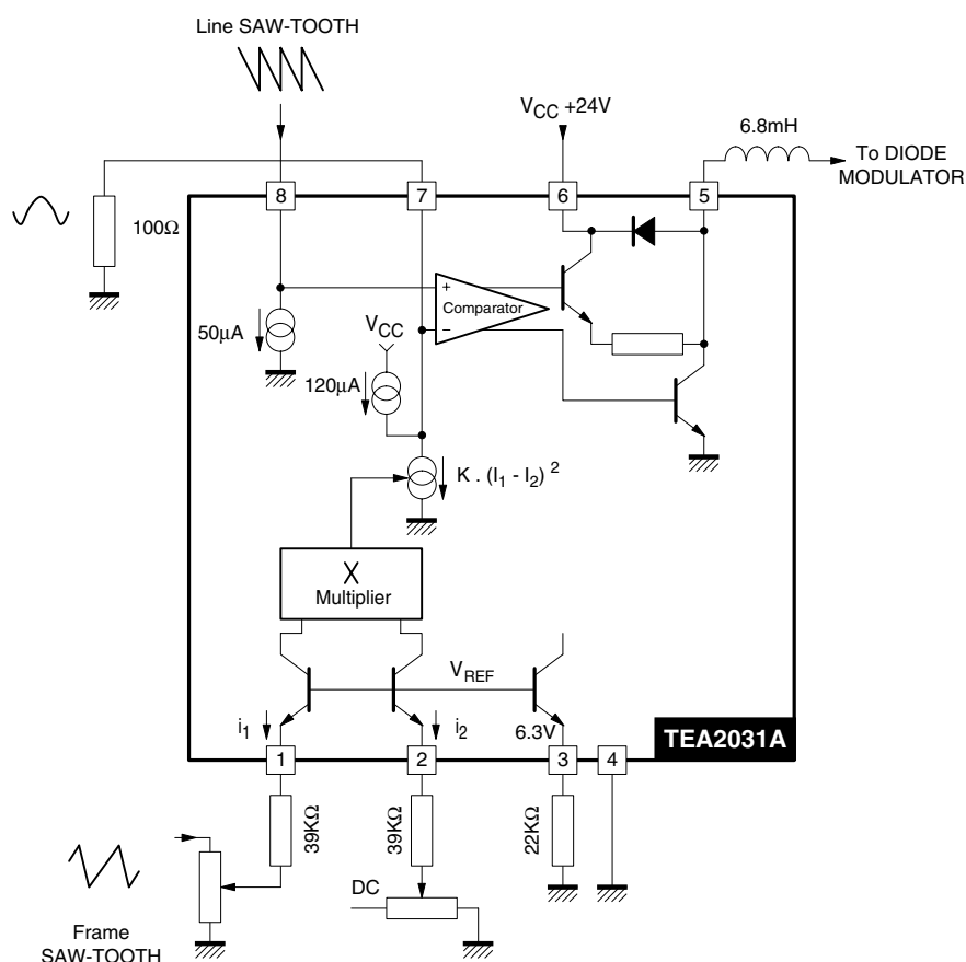
Figure 3. Block Diagram
