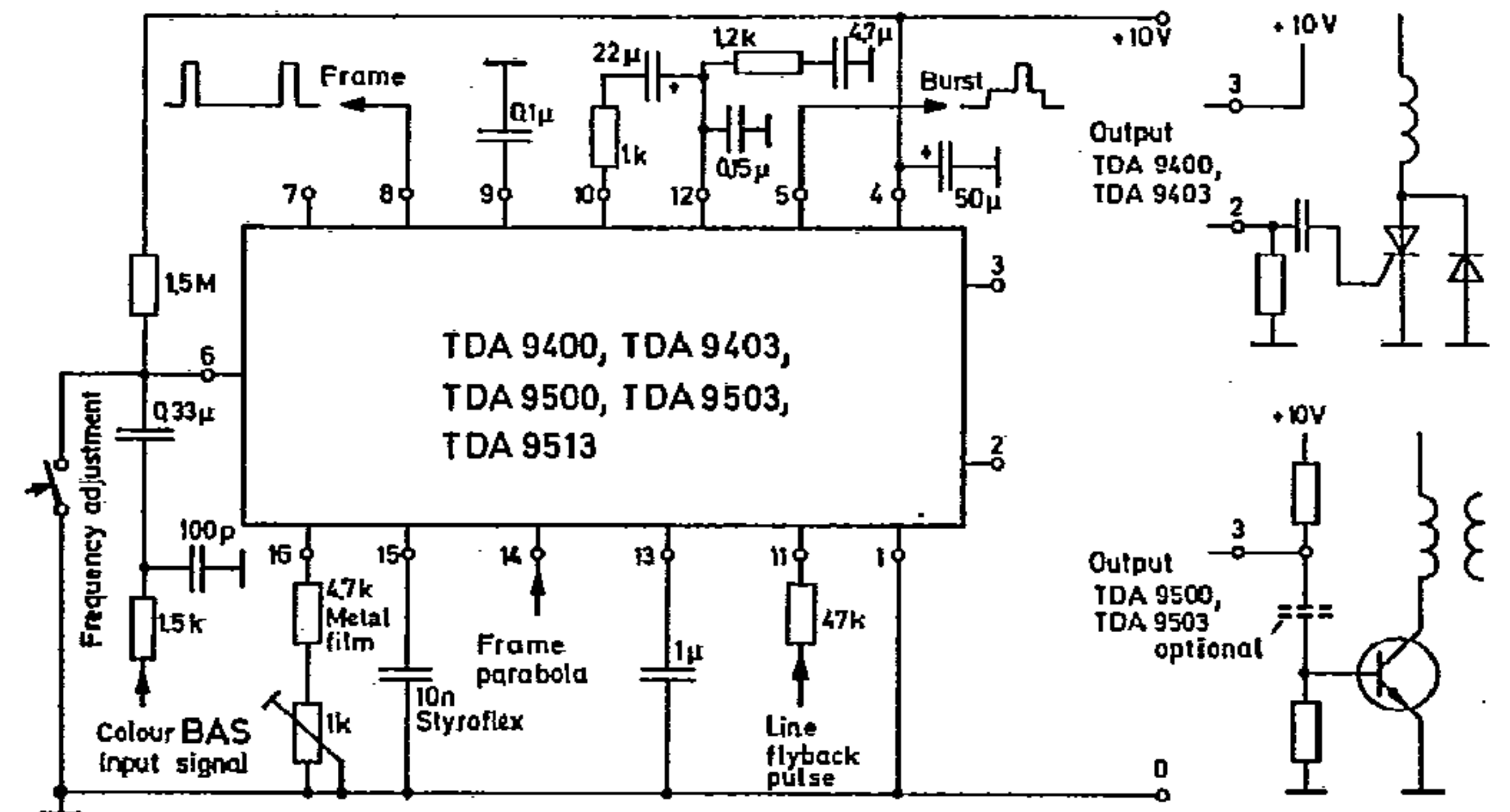
Application Circuit
