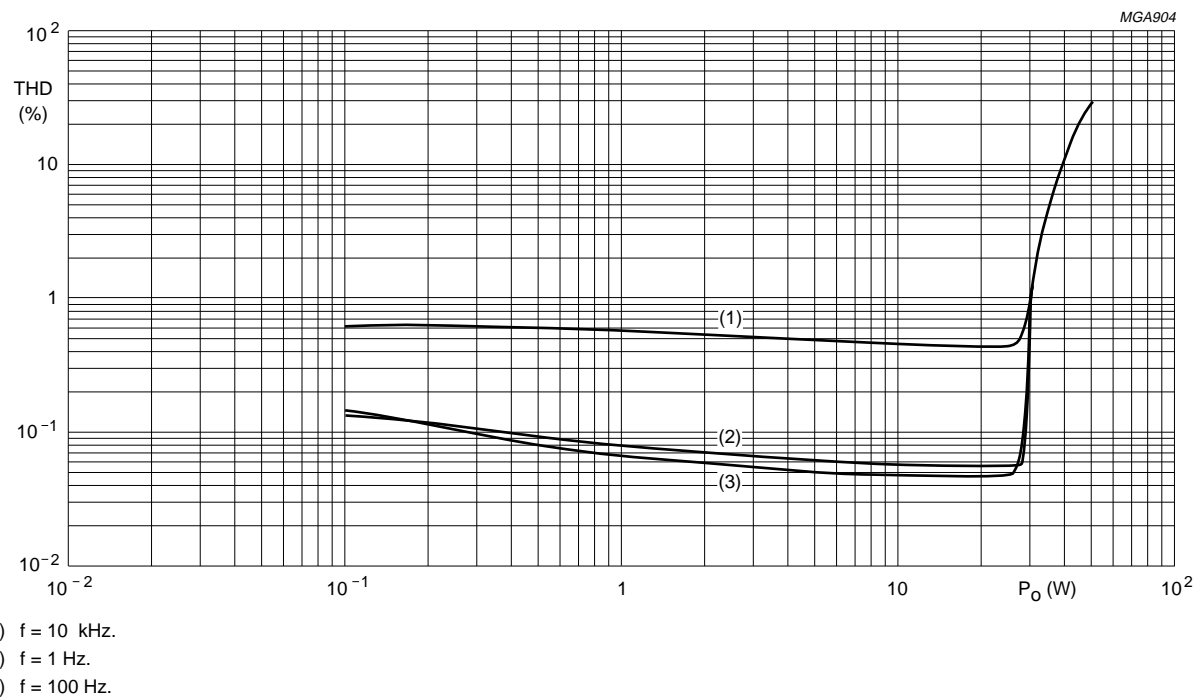
Fig.0 Total harmonic distortion as a function of output power; V_P = 14.4\text{ V} ; R_L = 2\text{ }\Omega .
