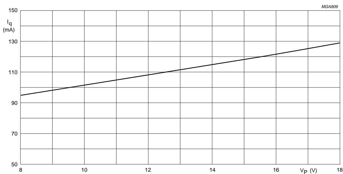
Fig.14 Quiescent current as a function of supply voltage; R_L = \infty .
