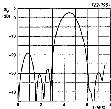
Fig.3 Typical frequency response of chrominance signal.
