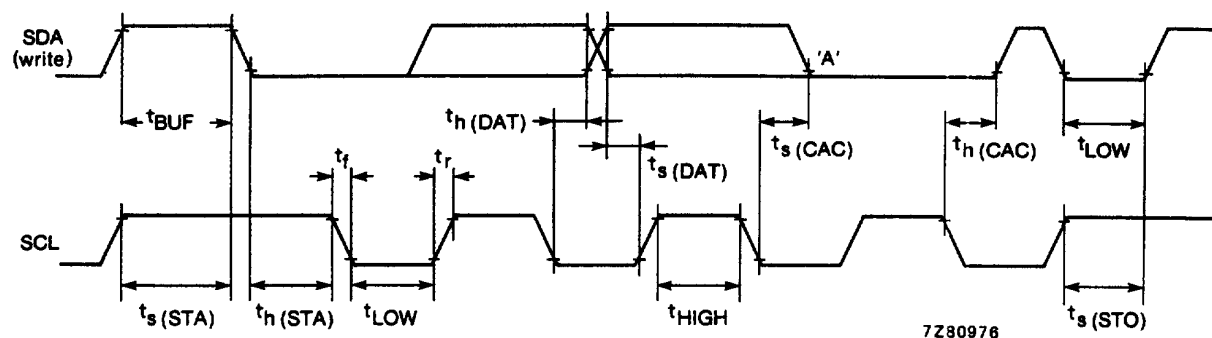
Fig.2 Timing diagram I²C bus.
