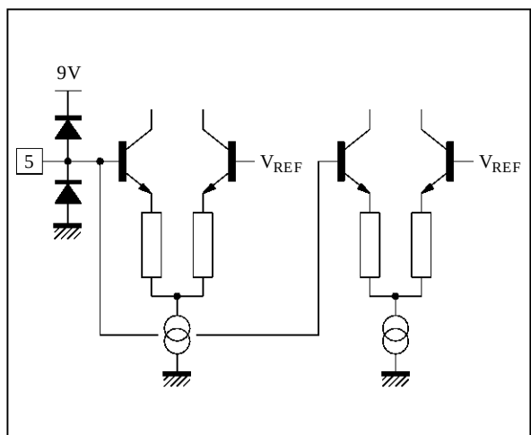
Figure 7 : Pin 5 Configuration
