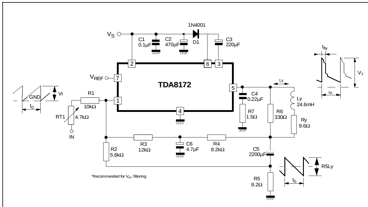
Figure 5. AC test circuit
