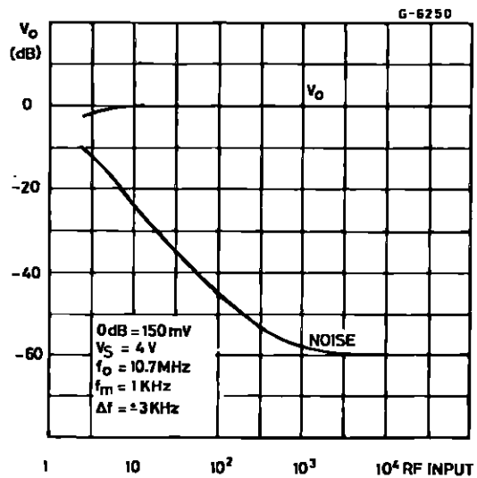
Figure 4 : FM IF Characteristics
