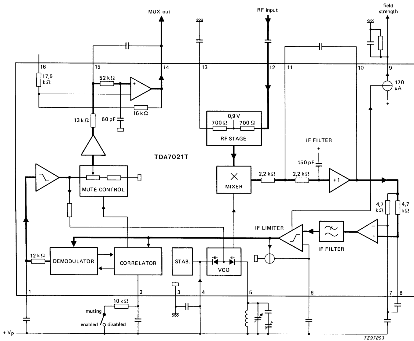
Fig.1 Block diagram.
