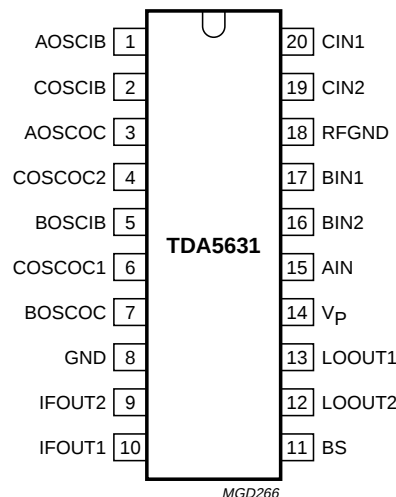
Fig.3 Pin configuration (TDA5631).
