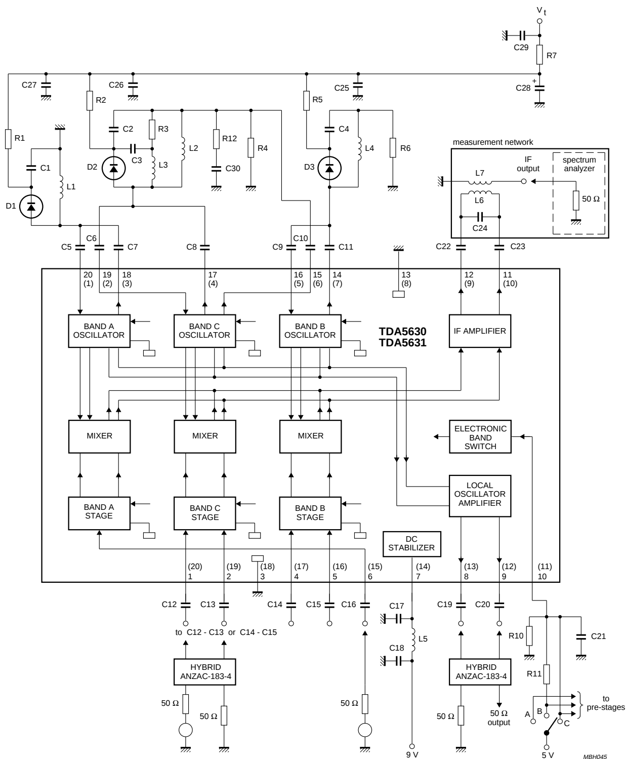
Fig.12 Measurement circuit.
