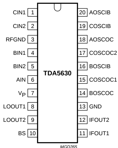
Fig.2 Pin configuration (TDA5630).
