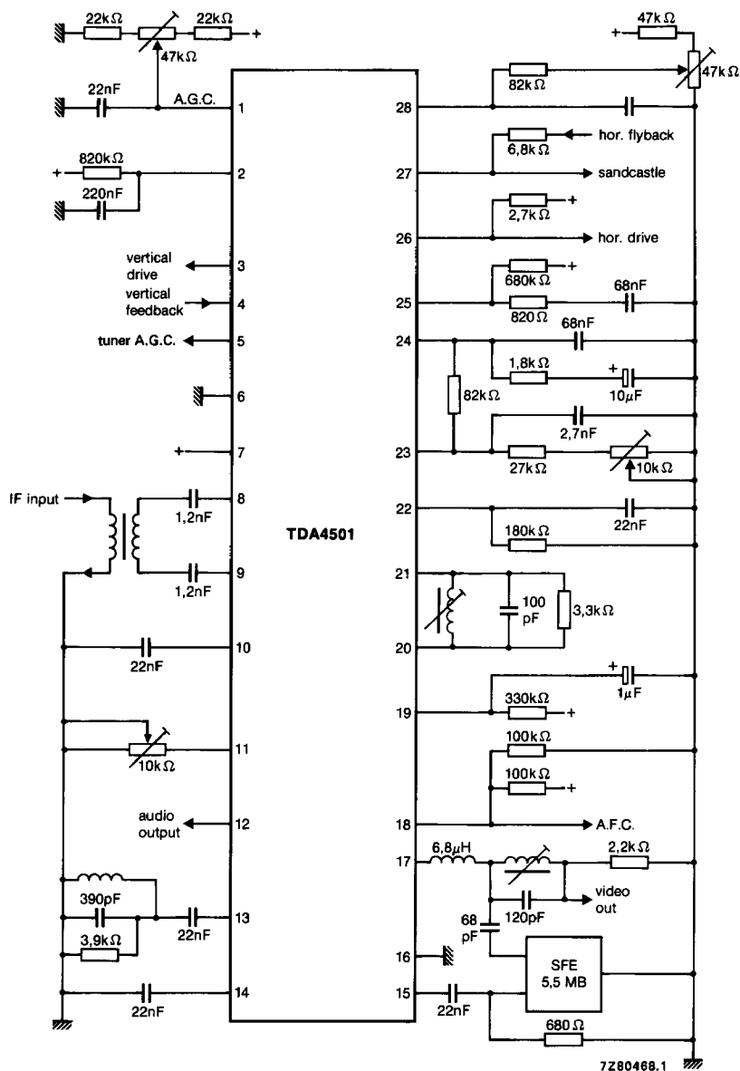
Fig. 2 Application diagram.
