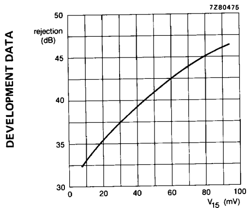
Fig. 9 AM rejection.
