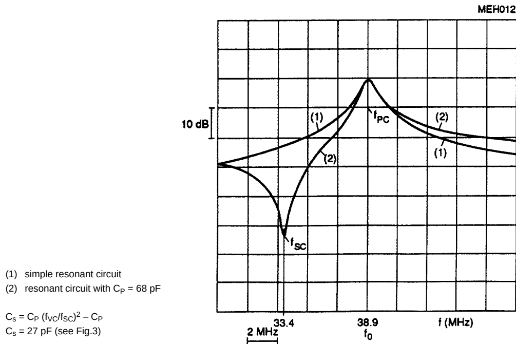
Fig.5 Frequency response of the 38.9 MHz reference circuit.
