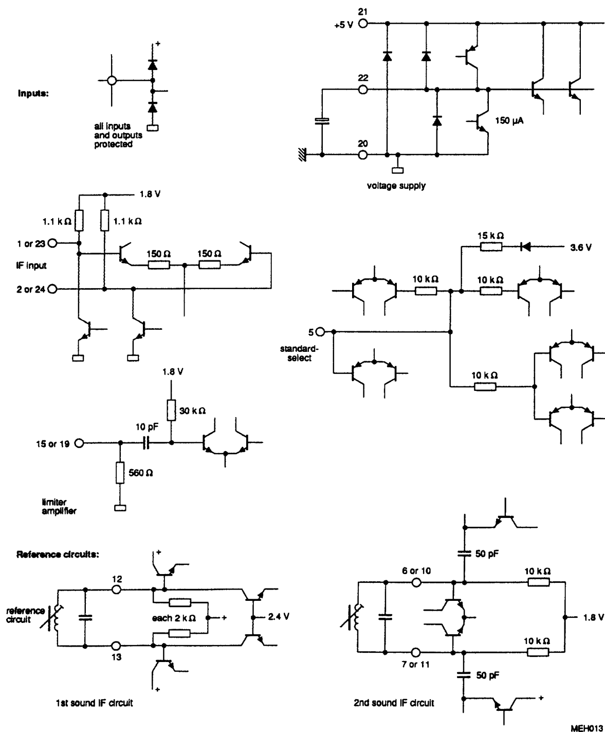
Fig.6 Internal circuits (continued in Fig.7).
