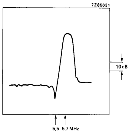
Fig. 5 IF2 filter selection.
