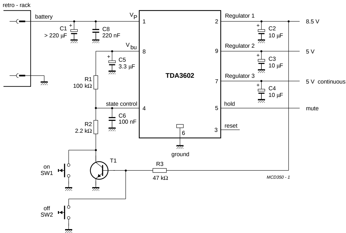
Fig.8 Application circuit 2.
