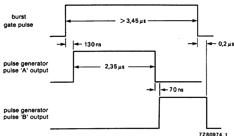
Fig.2 Burst gate timing pulse generation.
