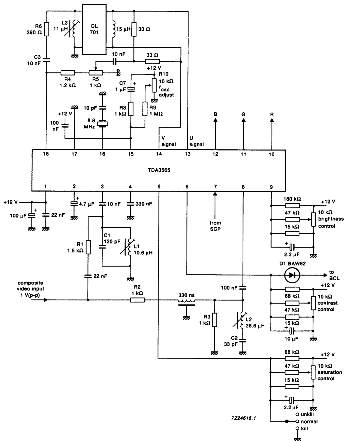
Fig.5 Application diagram
