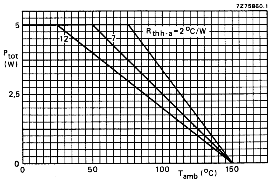
Fig.2 Total power dissipation. The graph takes into account an R_{\text{th} \text{tab-h}} = 1^{\circ}\text{C/W} which is to be expected when the tab is connected to a heatsink with one 3 mm bolt, without using heatsink compound. R_{\text{th} j\text{-tab}} = 12^{\circ}\text{C/W} .
