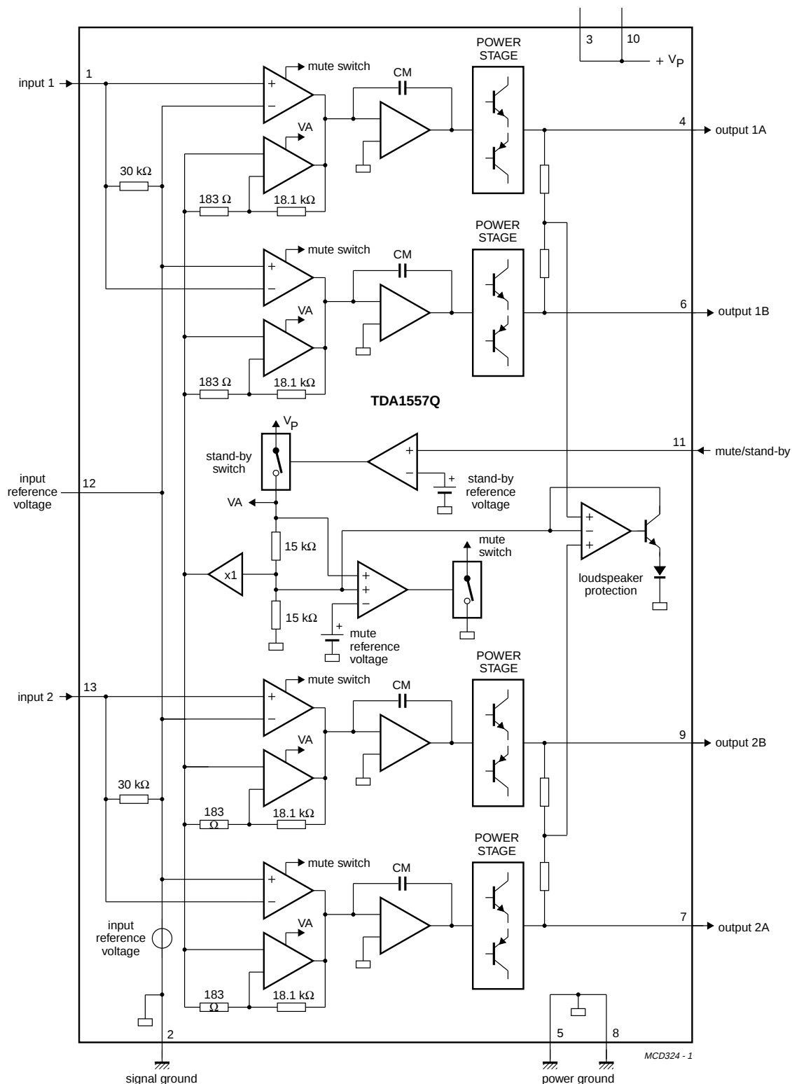
Fig.1 Block diagram.
