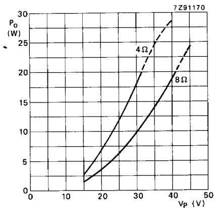
Fig. 3 Output power ( P_O ) as a function of supply voltage ( V_P ); f = 1 kHz; d_{tot} = 0.5\% ; G_V = 30 dB.
