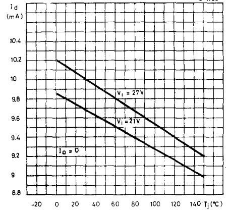
Typical quiescent drain current versus junction temperature
