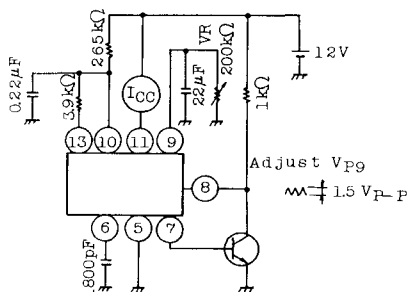
11. VERTICAL SUPPLY CURRENT
