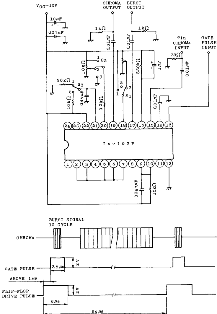
TEST CIRCUIT (1)
