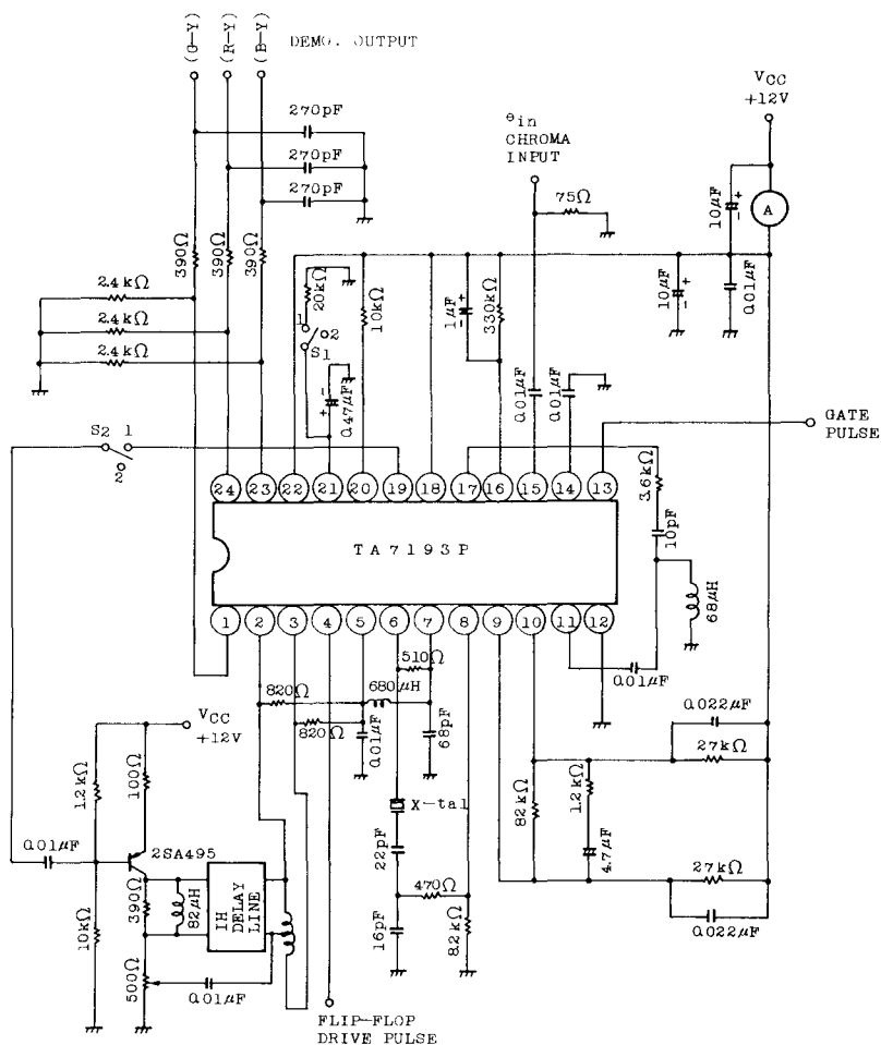
TEST CIRCUIT (4)
