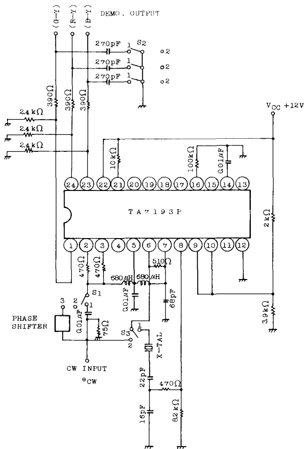
TEST CIRCUIT (3)
