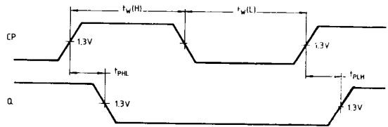
Fig. 1 Clock to Output Delays, Count Frequency, and Clock Pulse Width
