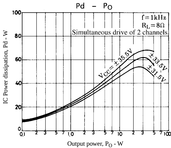
Figure 1. STK4182II Pd - PO ( R_L = 8\Omega )
