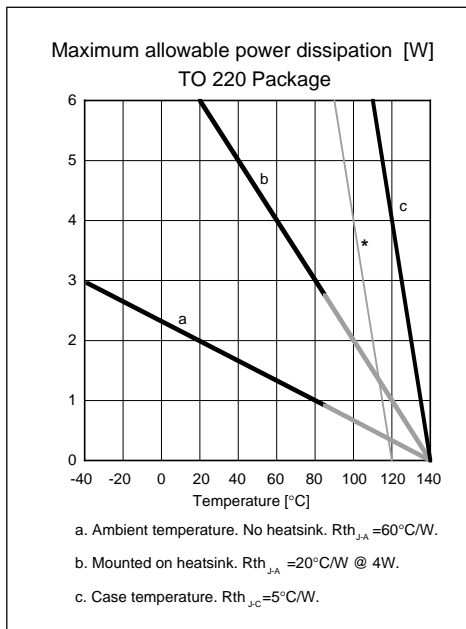
Figure 12. Maximum allowable power dissipation. TO 220 package
