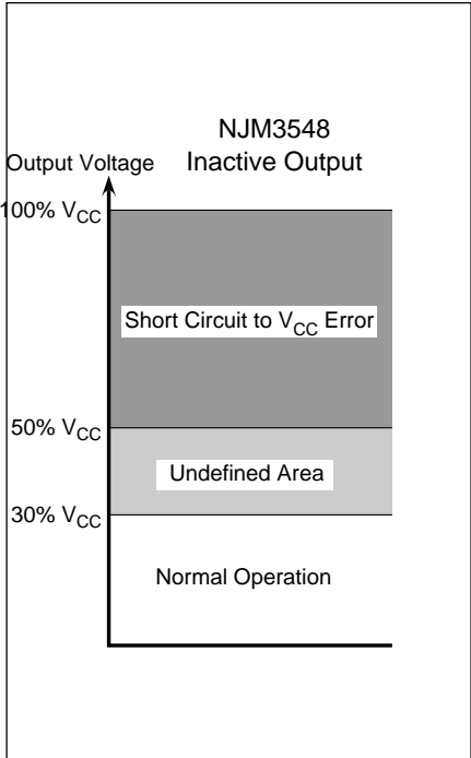
Figure 4. Error state vs. output voltage, inactive output ( 2.0 V \leq V_{IN} \leq V_{CC} , 5 V \leq V_{CC} \leq 40 V and -40^{\circ}C < T_J < +100^{\circ}C )
