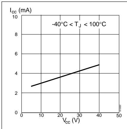
Figure 13. Current consumption vs. supply voltage at 2\text{ V} \leq V_{in} \leq V_{cc} V (Inactive output)
