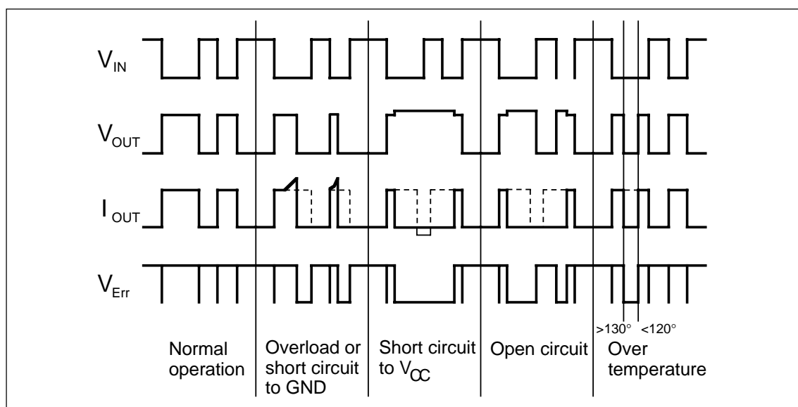
Figure 8. Signal diagram
