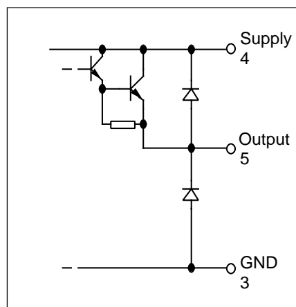
Figure 6. Output stage
