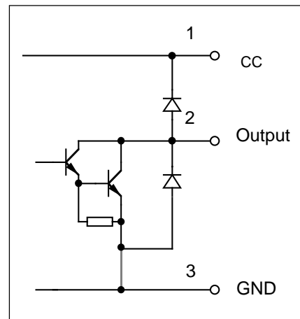
Figure 6. Output stage
