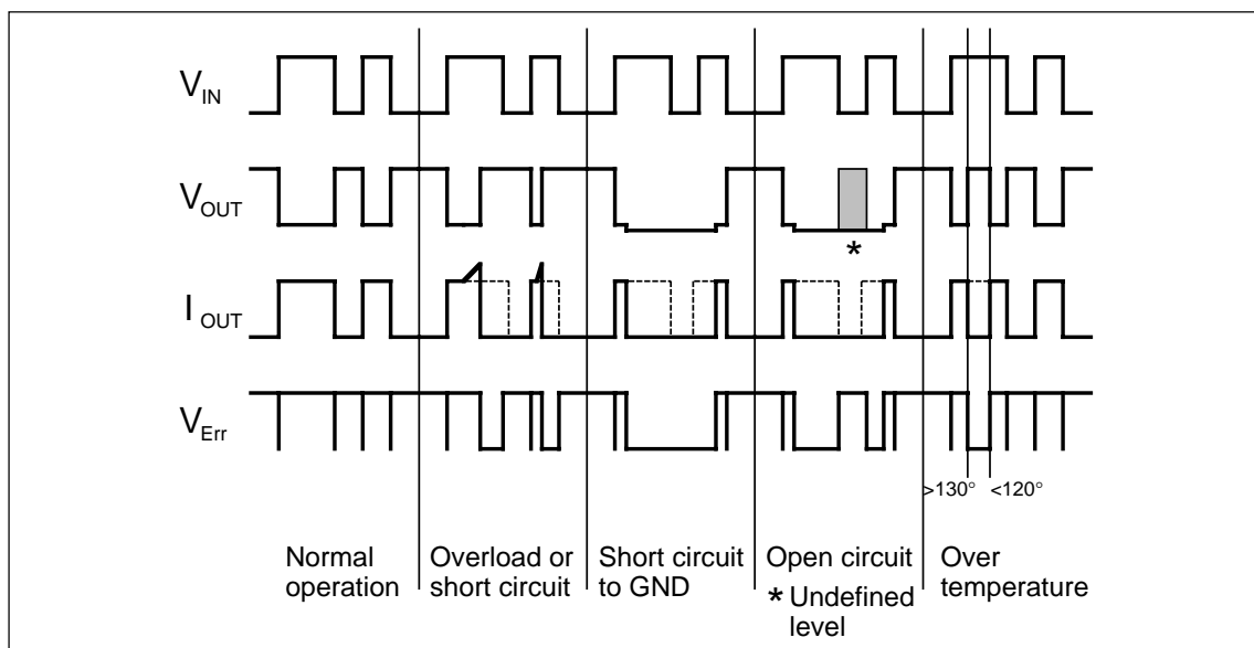
Figure 8. Signal diagram
