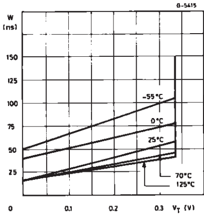
Figure 1 : Minimum Pulse Width Required for Trigning
