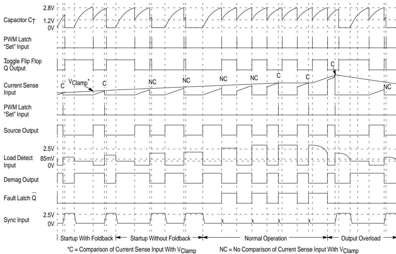
Figure 28. Timing Diagram
