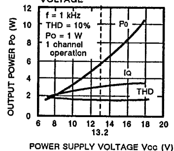
Fig. 6 — OUTPUT POWER/TOTAL HARMONIC DISTORTION/QUIESCENT POWER SUPPLY CURRENT vs. POWER SUPPLY VOLTAGE
