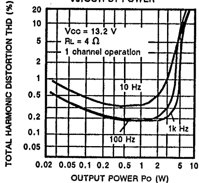
Fig. 4 — TOTAL HARMONIC DISTORTION vs. OUTPUT POWER
