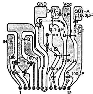
Fig. 3 — TYPICAL APPLICATION CIRCUIT PATTERN (BOTTOM VIEW)
