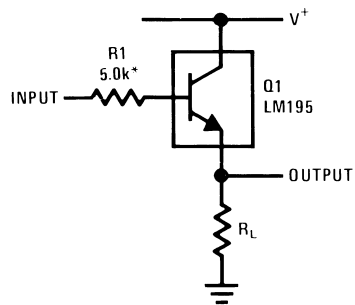
Emitter Follower
