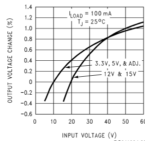
Line Regulation
