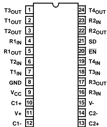
HIN236 (SOIC) TOP VIEW
