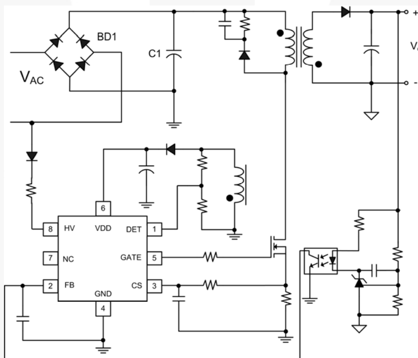
Figure 1. Typical Application
