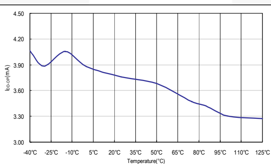
Figure 9. Operating Current
