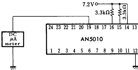
Test Circuit 11 ( I_{IL(SK)} )
