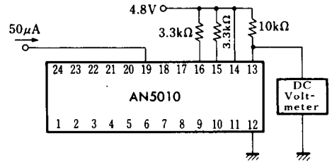
Test Circuit 12 ( I_{IH(SK)} )
