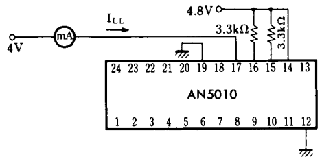
Test Circuit 14 ( I_{IH(OS)} )
