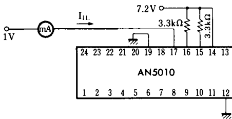
Test Circuit 13 ( I_{IL(OS)} )
