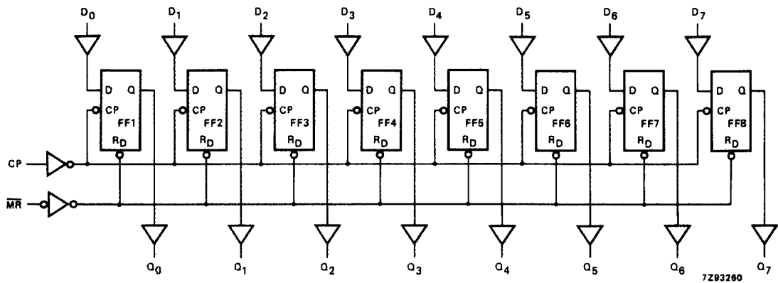
Fig.5 Logic diagram.
