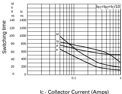
Switching Speeds
