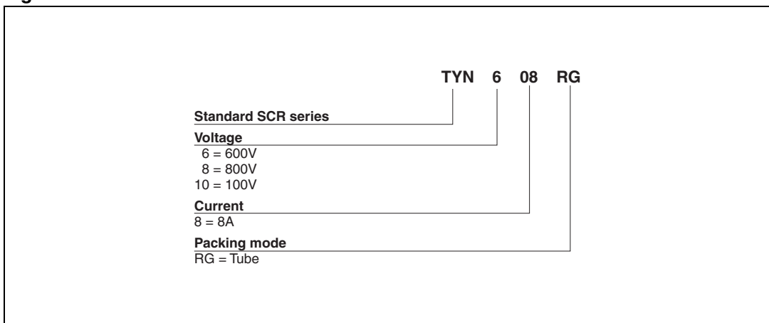
Figure 17. TYNx08 series
