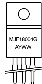
TO-220 FULLPACK CASE 221D STYLE 2 UL RECOGNIZED
