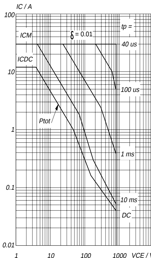
Fig.15. Forward bias safe operating area. T_{hs} = 25^\circ\text{C} I_{CDC} \& I_{CM} = f(V_{CE}) ; I_{CM} single pulse; parameter t_p Second-breakdown limits independent of temperature. Mounted with heatsink compound.
