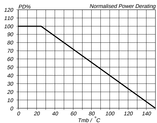
Fig.15. Normalised power dissipation. PD\% = 100 \cdot P_D / P_{D\ 25^\circ\text{C}} = f(T_{mb})
