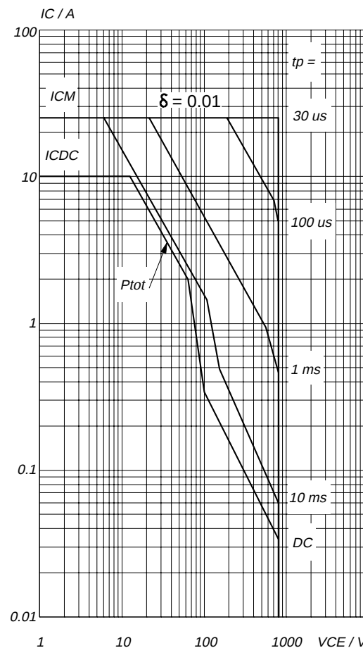
Fig.17. Forward bias safe operating area. T_{mb} = 25^\circ\text{C} I_{CDC} & I_{CM} = f(V_{CE}) ; I_{CM} single pulse; parameter t_p Second-breakdown limits independent of temperature.
