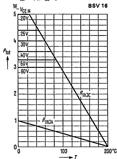
Total perm. power dissipation versus temperature P_{\text{tot}} = f(T); V_{CE} = \text{parameter}
