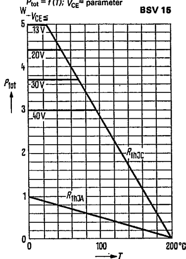
Total perm. power dissipation versus temperature P_{\text{tot}} = f(T); V_{CE} = \text{parameter}
