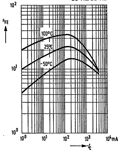
DC current gain h_{FE} = f(I_C) V_{CE} = 1\text{V} ; T_{case} = \text{parameter} BD 434, BD 436, BD 438, BD 440, BD 442
