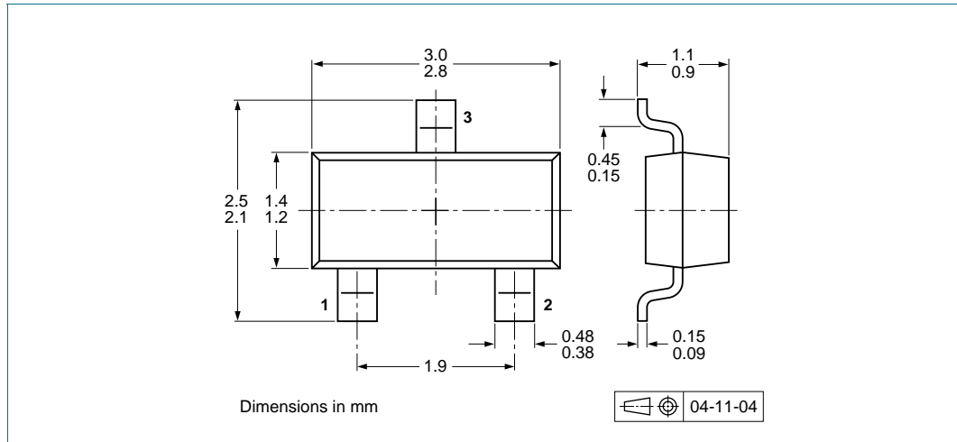
Fig 9. Package outline SOT23 (TO-236AB)
